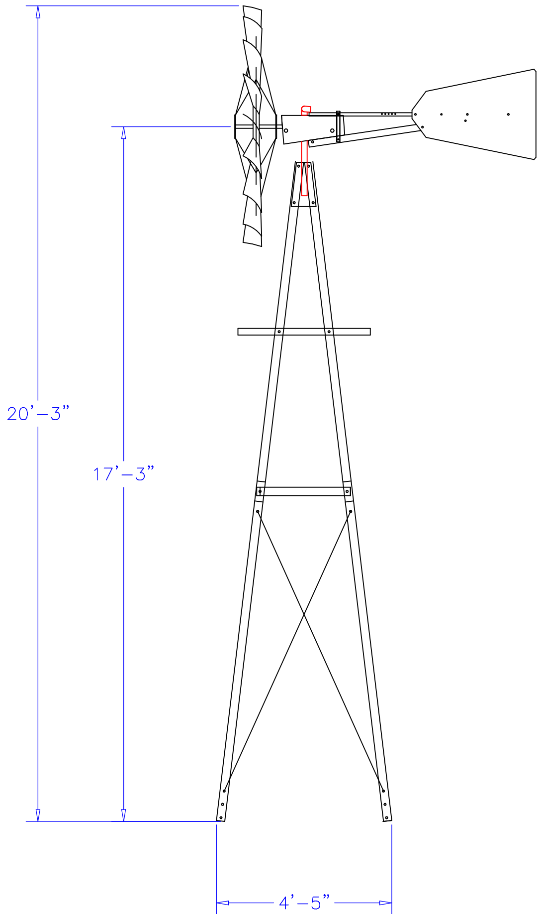
16' TOWER WITH 6' FAN
