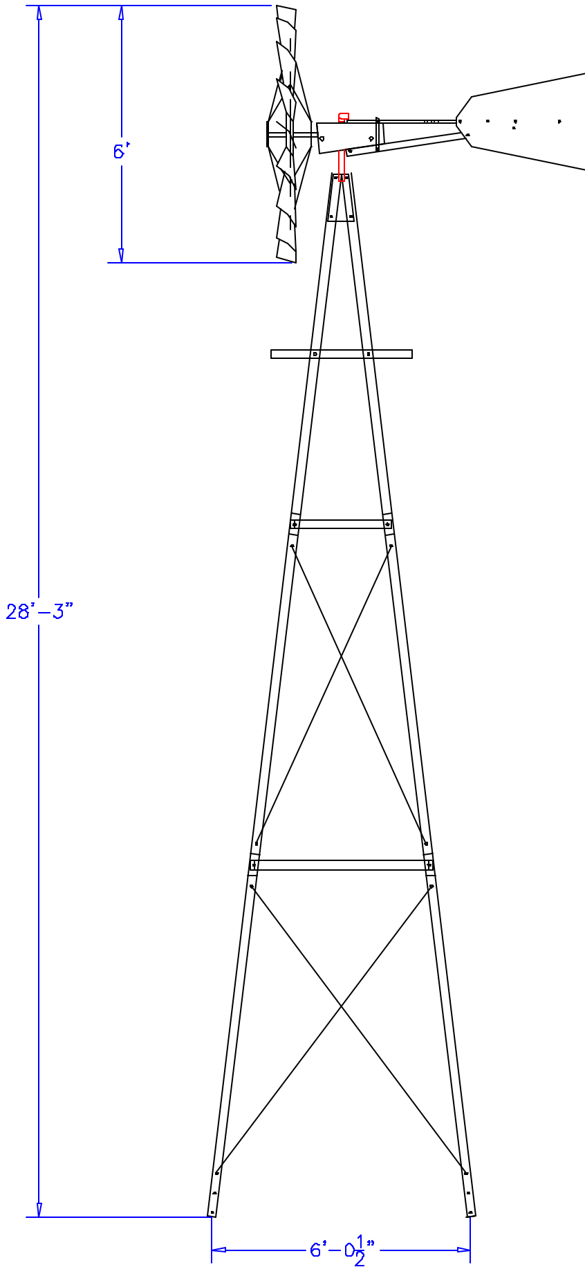
24' TOWER WITH 6' FAN
